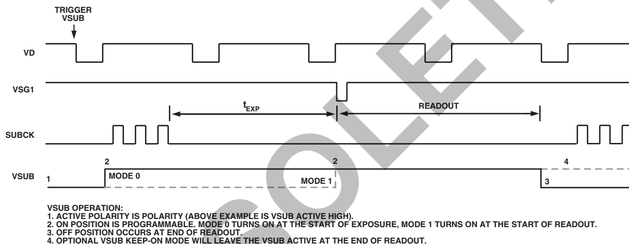
Figure 29. VSUB Programmability
