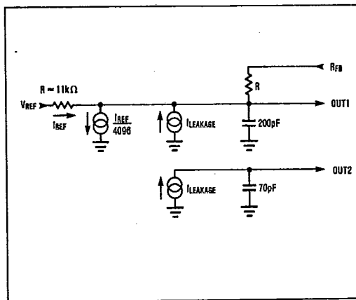
Figure 3. AD7541A DAC Equivalent Circuit, All Digital Inputs HIGH
