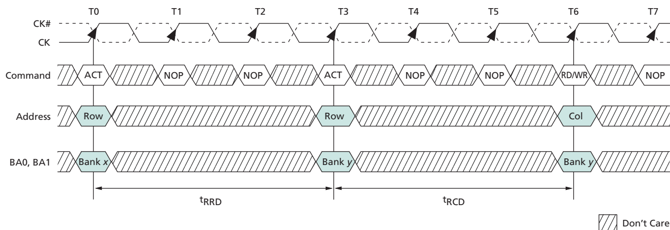
Figure 27: Example: Meeting t_{\text{RCD}} ( t_{\text{RRD}} ) MIN When 2 < t_{\text{RCD}} (t_{\text{RRD}}) \text{ MIN} / t_{\text{CK}} \leq 3
