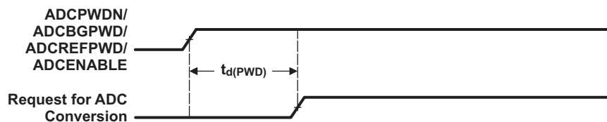
Figure 6-19. ADC Conversion Timing
