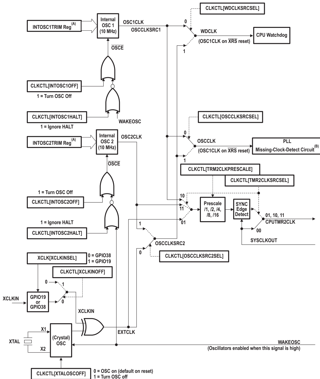
Figure 6-8. Clock Tree
