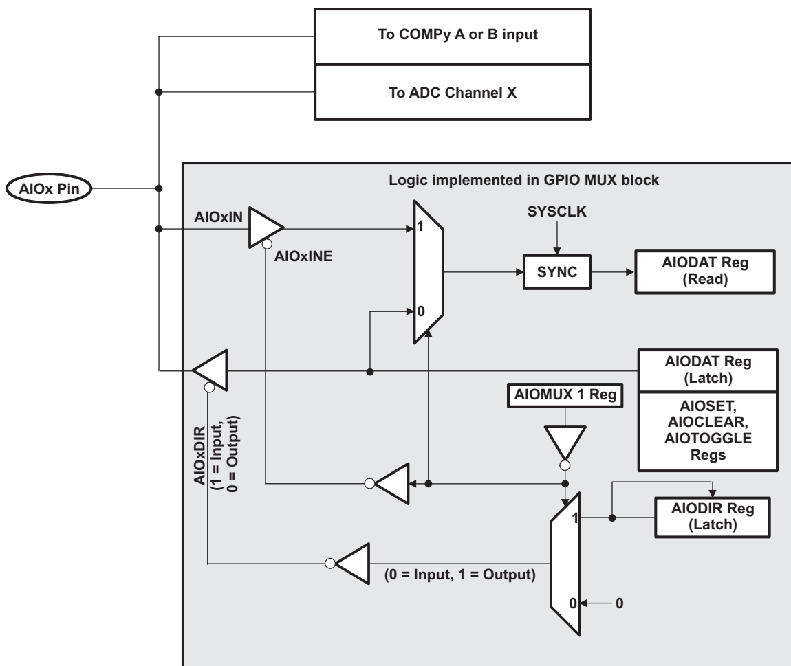
Figure 6-25. AlOx Pin Multiplexing
