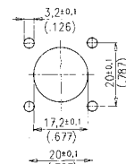
Panel Cutout
