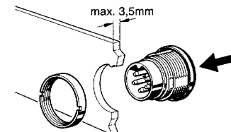
Assembling instruction
