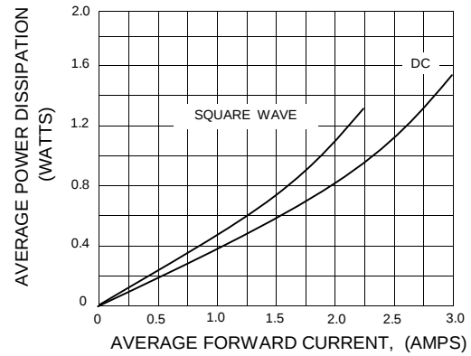
FIG.2 - FORWARD POWER DISSIPATION
