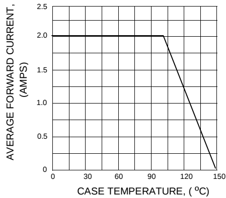
FIG.1 - CURRENT DERATING
