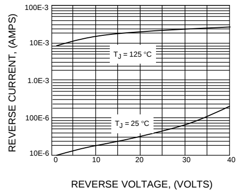
FIG.4 - TYPICAL REVERSE CURRENT
