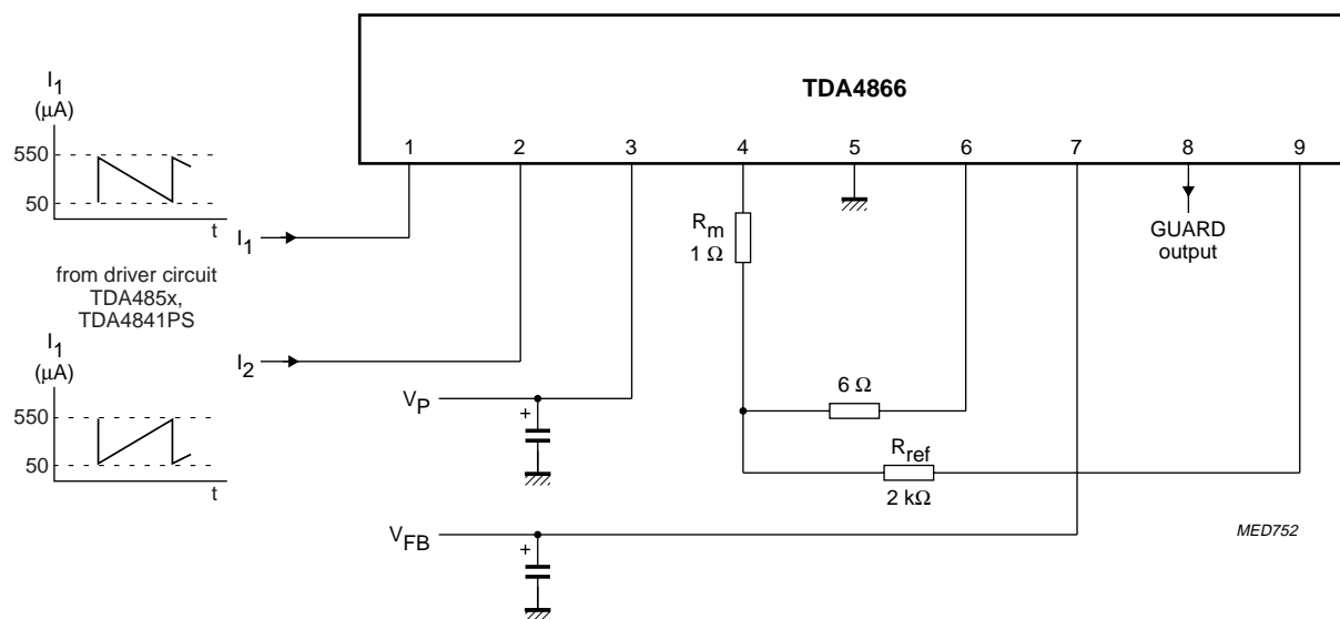
Fig.6 Test diagram.
