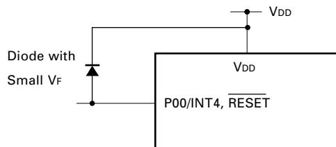
○ Diode connected between P00/INT4 or \overline{\text{RESET}} and V_{DD}
