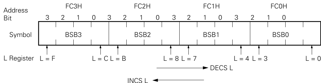
Fig. 5-8 Bit Sequential Buffer Format
