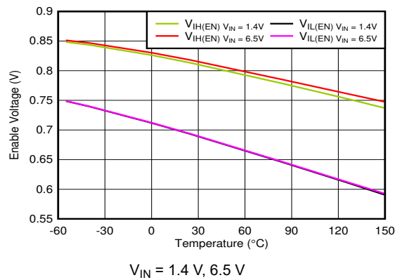
Figure 6-85. Enable Threshold vs Temperature
