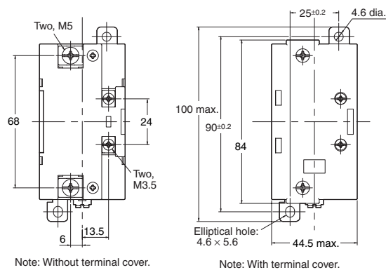
Mounting Holes
