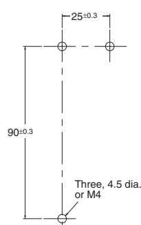
Mounting Holes
