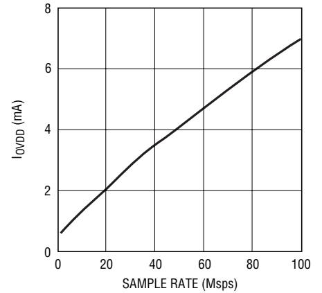
LTC2233: I_{VDD} vs Sample Rate, 5MHz Sine Wave Input, -1\text{dB} , 0V_{DD} = 1.8V
