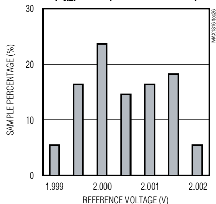
REFERENCE VOLTAGE DISTRIBUTION ( V_{REF} = 2.0V , SAMPLE SIZE = 55)
