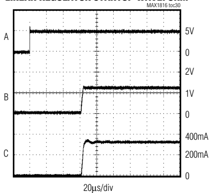
LINEAR REGULATOR STARTUP WAVEFORM
