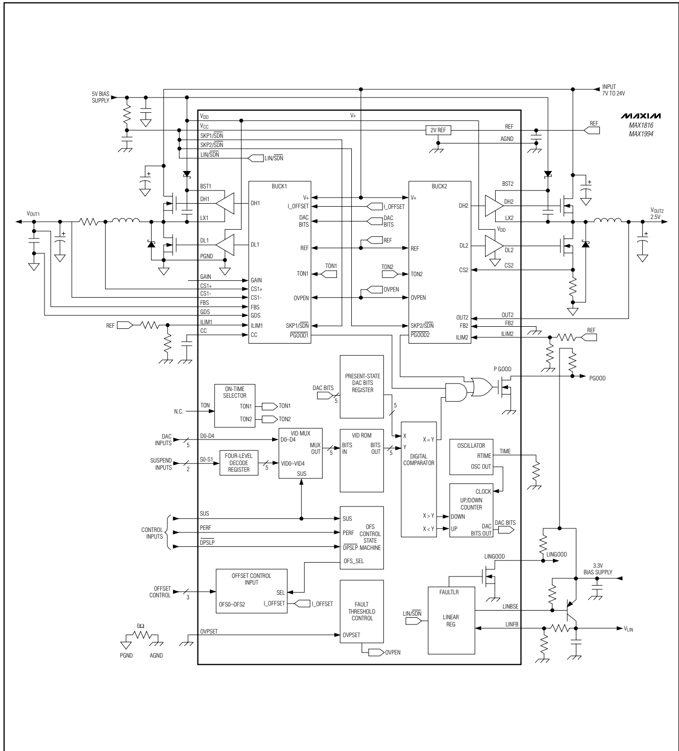
Figure 3. Functional Diagram
