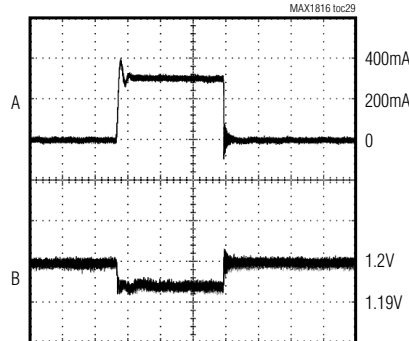
LINEAR REGULATOR LOAD TRANSIENT RESPONSE
