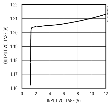
LINEAR REGULATOR LINE REGULATION
