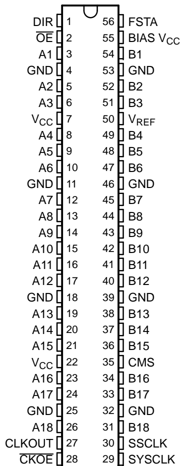
DGG OR DGV PACKAGE (TOP VIEW)
