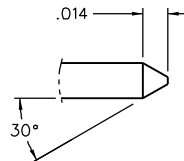
POINTING DETAIL 20:1
