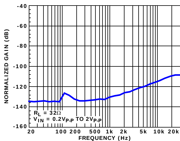
FIGURE 13. OFF-ISOLATION
