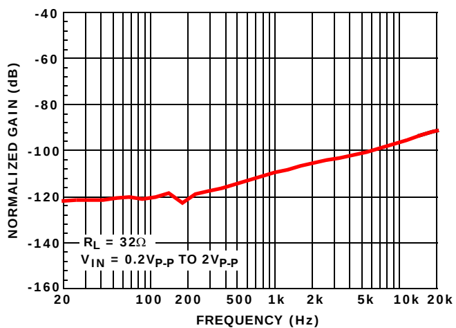
FIGURE 14. CROSSTALK
