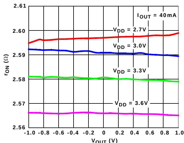
FIGURE 6. ON-RESISTANCE vs SWITCH VOLTAGE vs SUPPLY VOLTAGE
