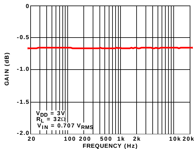
FIGURE 12. INSERTION LOSS
