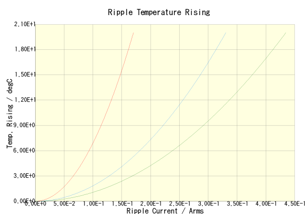
C1608X8R1H223K080AA(100kHz) C1608X8R1H223K080AA(500kHz) C1608X8R1H223K080AA(1MHz)
