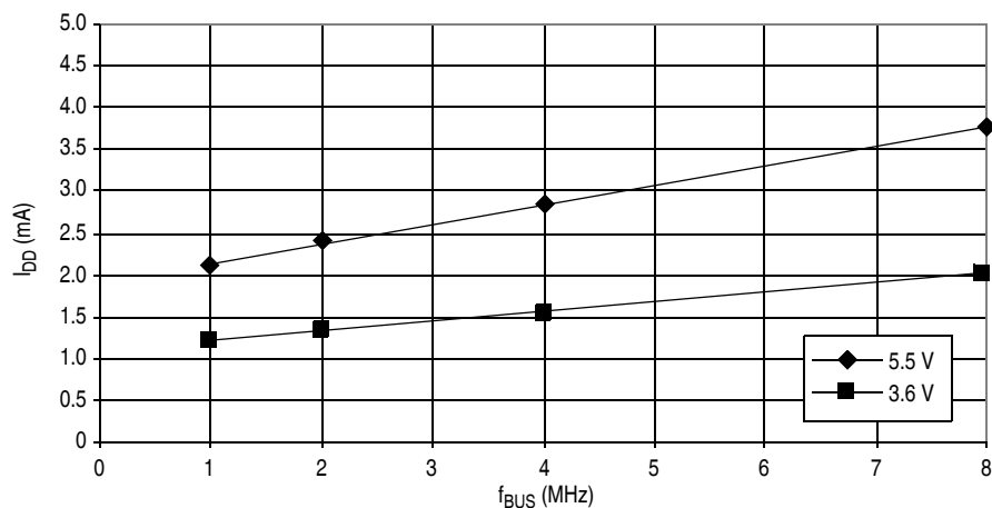
Figure 20-16. Typical Wait Mode I_{\text{DD}} , with all Modules Disabled ( -40^{\circ}\text{C} to 85^{\circ}\text{C} )
