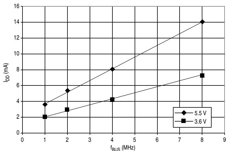
Figure 20-15. Typical Operating I_{\text{DD}} , with All Modules Turned On ( -40^{\circ}\text{C} to 85^{\circ}\text{C} )
