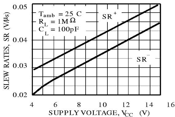
Figure 9 : Slew Rate versus Supply Voltage
