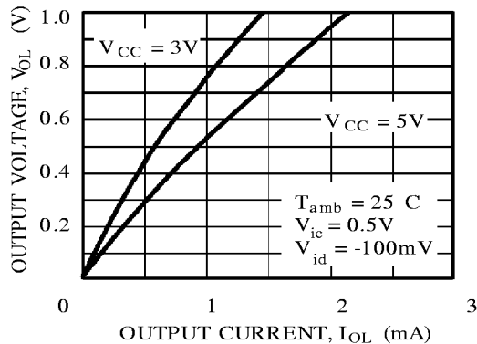
Figure 3a : Low Level Output Voltage versus Low Level Output Current
