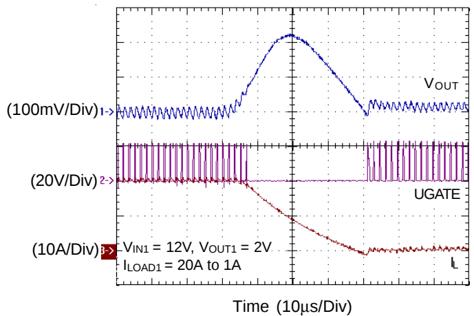
Transient Response
