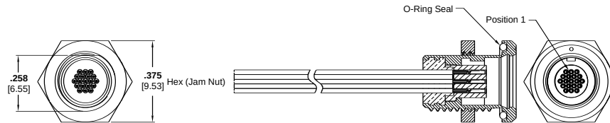
19 Position Drawing Number 1589058
