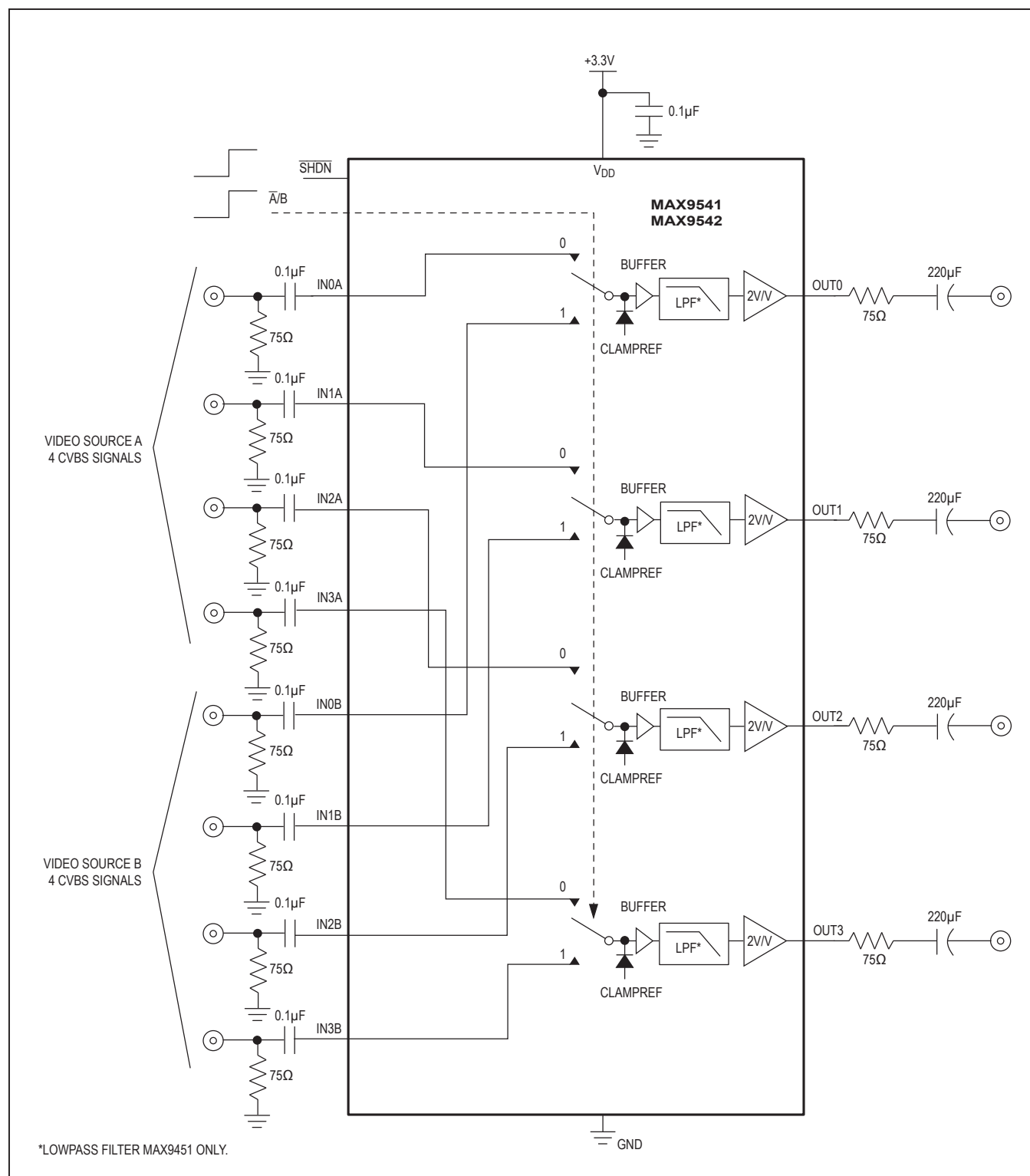
Figure 3. AC-Coupled Outputs
