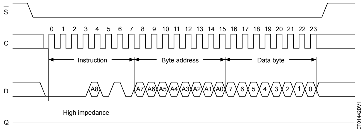
Figure 11. Byte write (WRITE) sequence
