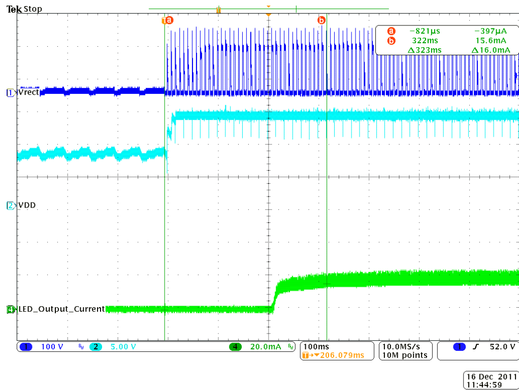
Figure 24. ILED at Minimum Dim Angle, Turn-on Waveforms
