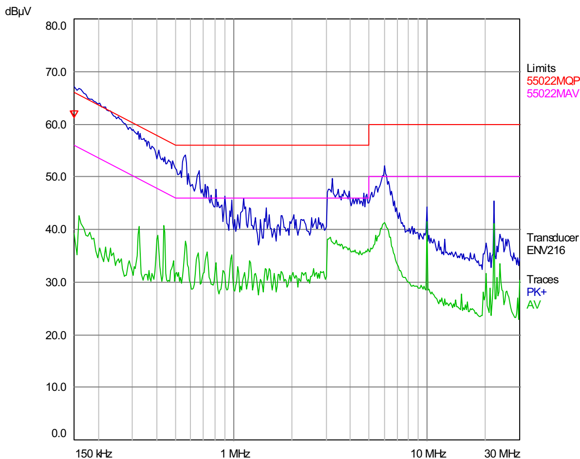
Figure 25. Conducted EMI
