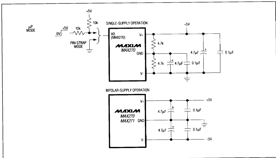
Figure 4. Power-Supply Configurations
