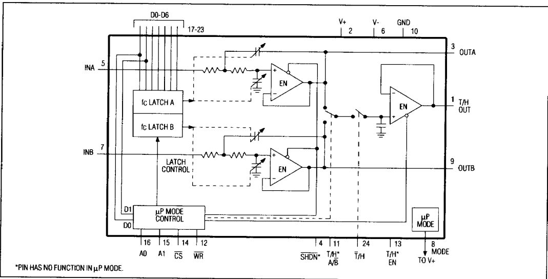
Figure 1b. MAX271 Block Diagram - \mu P Mode
