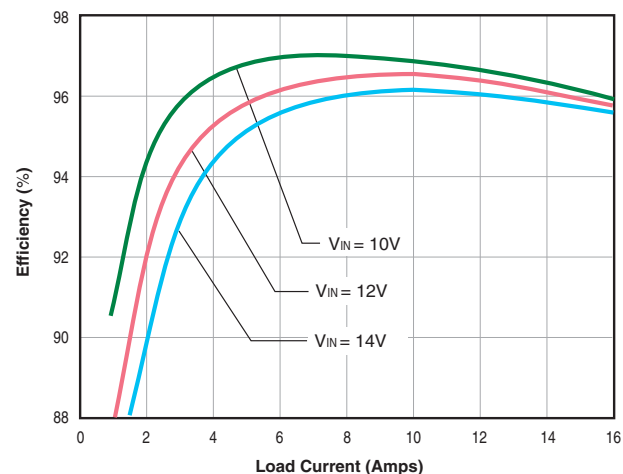
Efficiency vs. Line Voltage and Load Current @ 25°C
