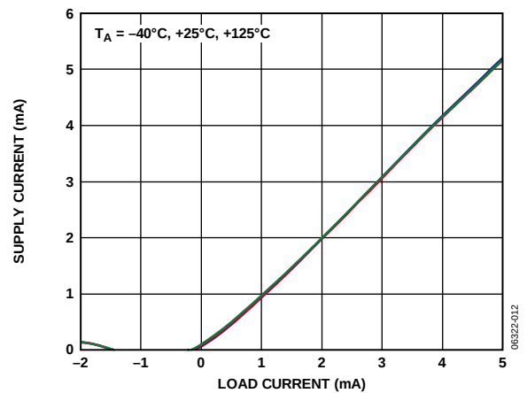
Figure 12. Supply Current vs. Load Current, V_{OUT} = 1\text{ V}
