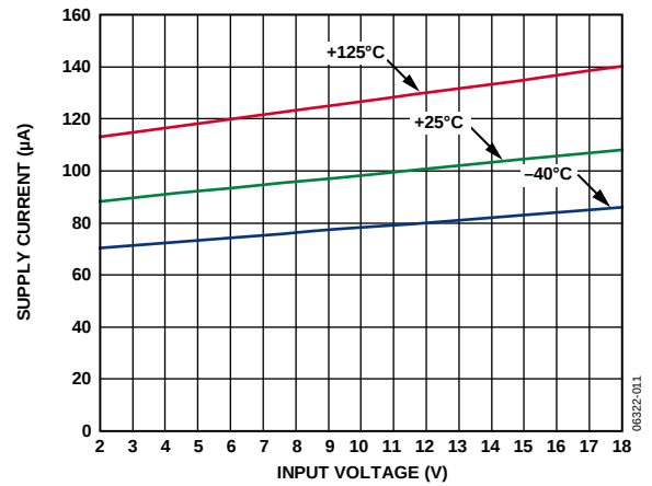
Figure 11. Supply Current vs. Input Voltage, V_{OUT} = 1\text{ V}
