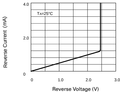
Reverse Characteristics
