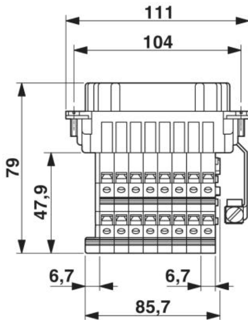
Dimensioned drawing
