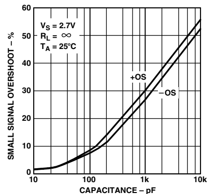
Figure 9. Small Signal Overshoot vs. Load Capacitance
