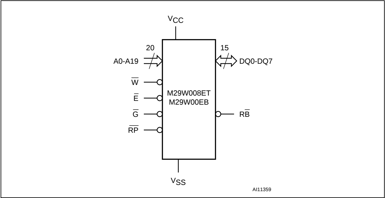
Figure 2. Logic diagram
