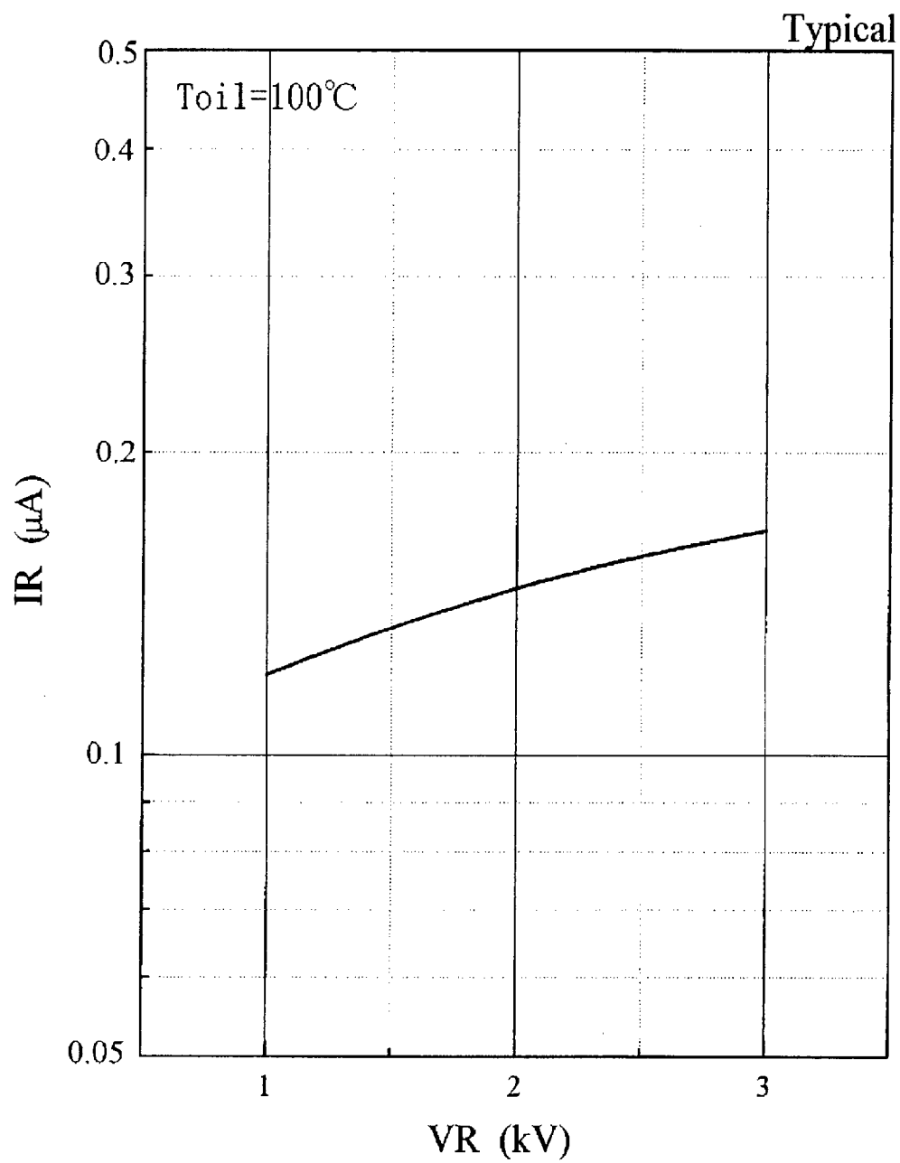
Fig.2 Reverse characteristic[VR-IR]
