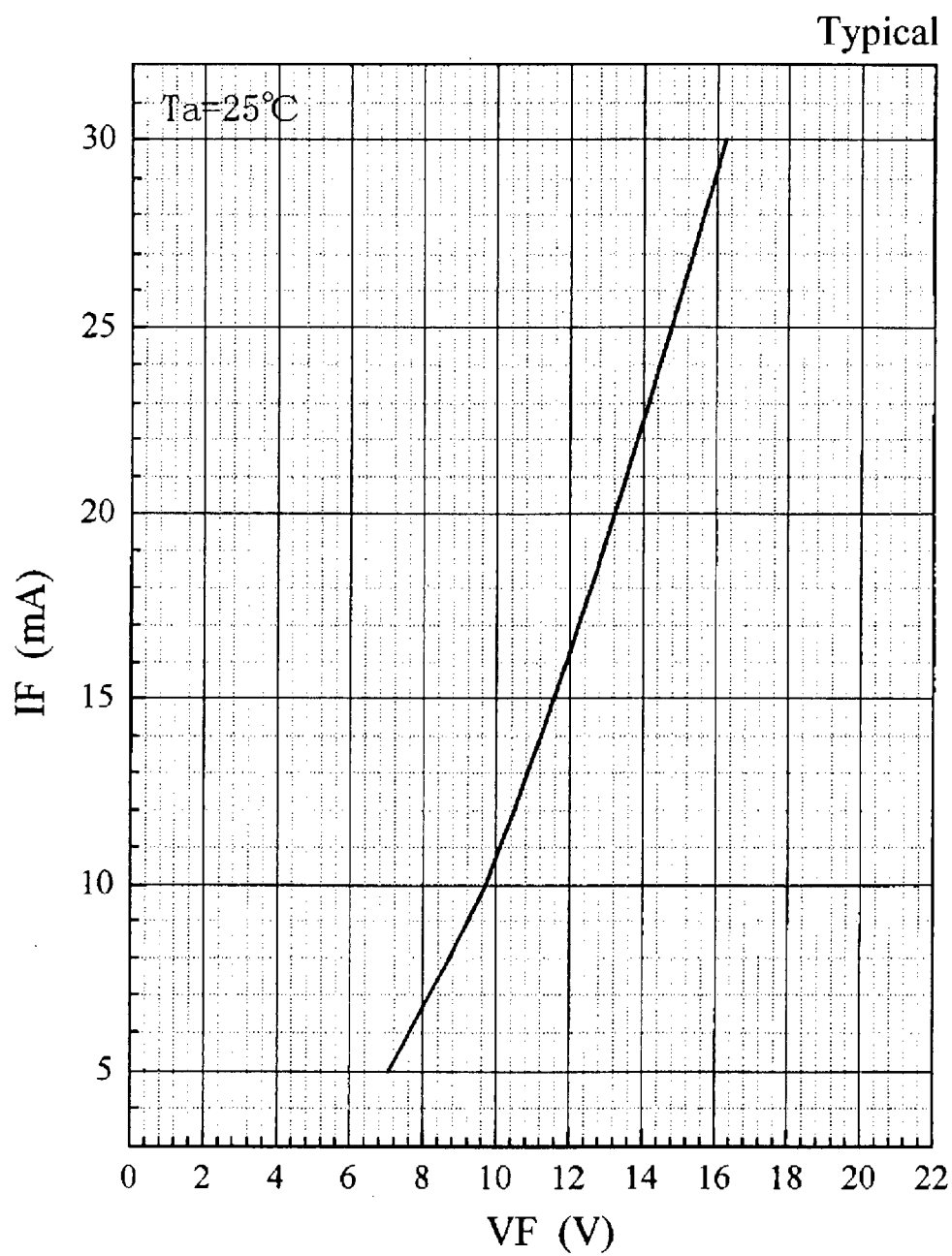
Fig.1 Forward characteristic[ V_F - I_F ]
