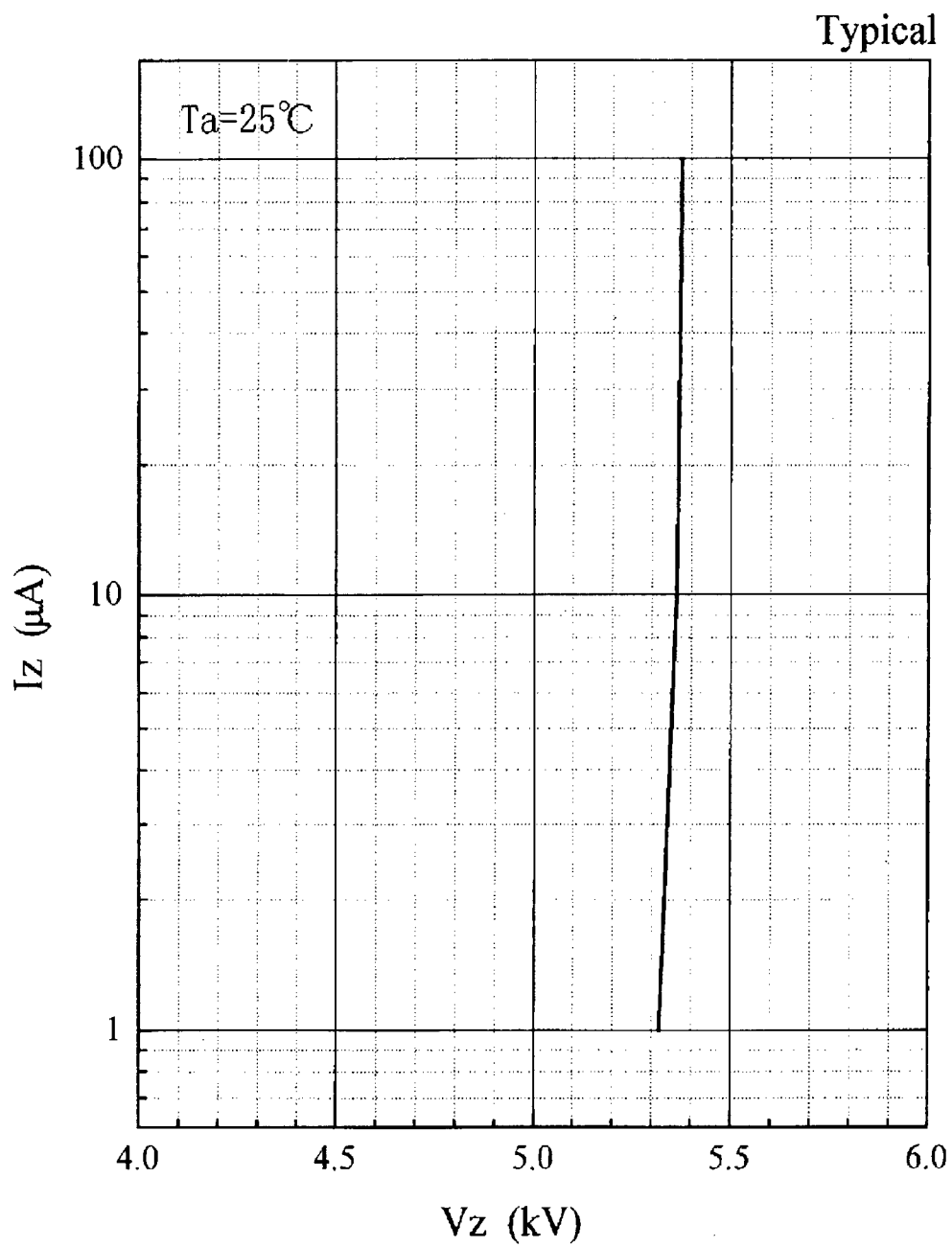
Fig.3 Avalanche characteristic [ V_z - I_z ]
