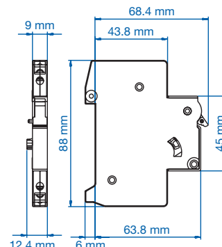
Dimensions HLS11L.
