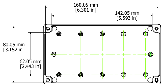
BOX - INSIDE
