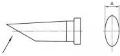
Soldering tip LT DD 45°, 4,6 mm, packed 10 pcs.
