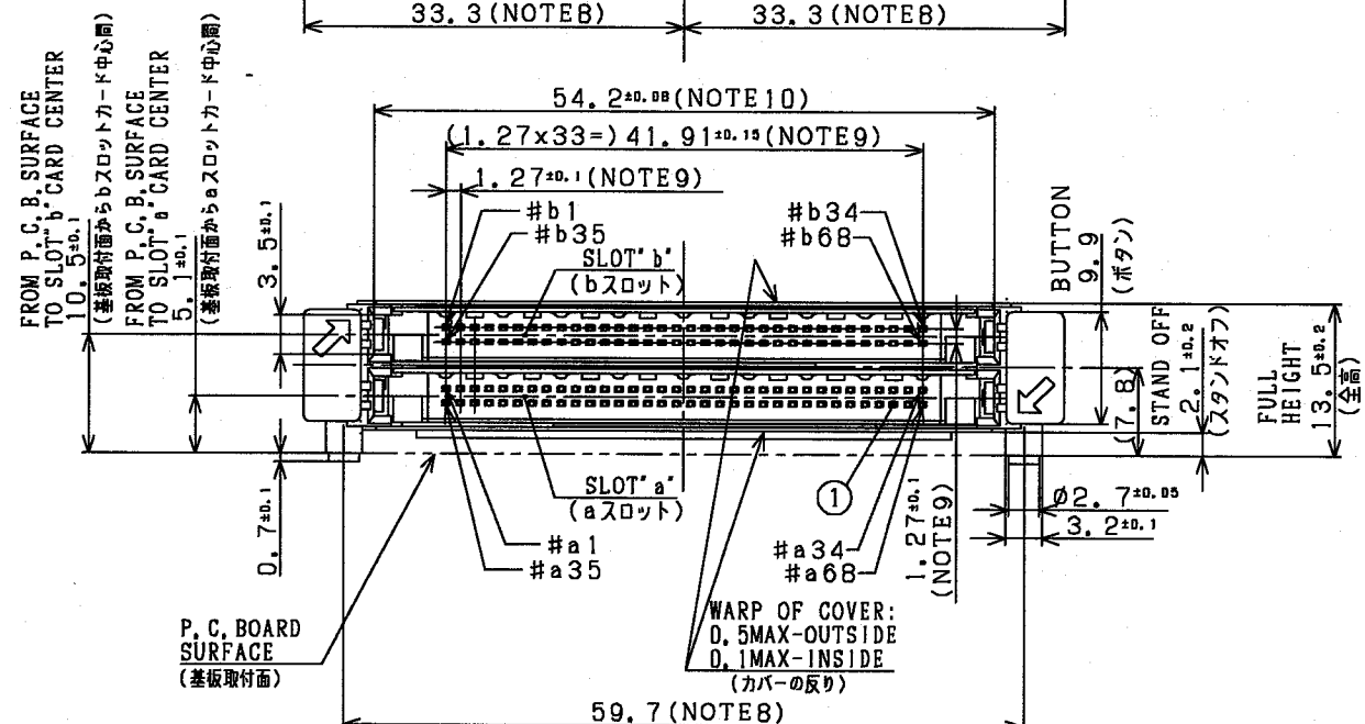
PIN # (タシシ番号) L (mm) a1, a17, a34, a35, a51, a68 b1, b17, b34, b35, b51, b68 5.00±0.1 a36, a67, b36, b67 3.50±0.1 OTHER (上記以外) 4.25±0.1
