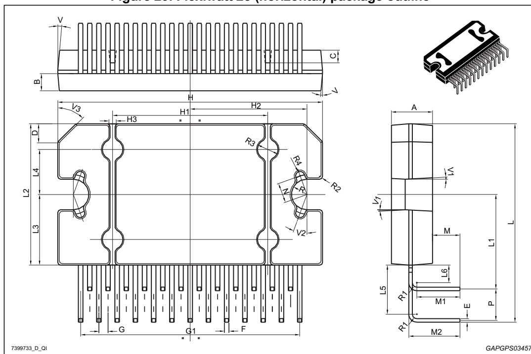
Figure 29. Flexiwatt 25 (horizontal) package outline
