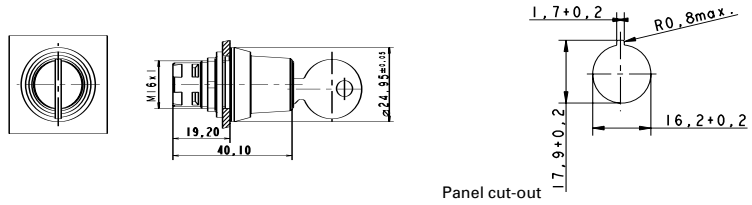
Panel cut-out
