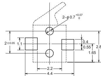
PCB mounting hole and land dimensions (Reference) (View from switch top)
