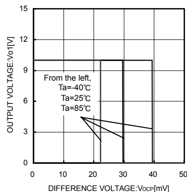
Fig.12 External OCP Detection Voltage
