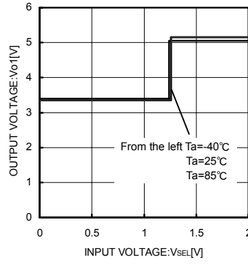
Fig.17 SEL Threshold Voltage
