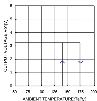
Fig.9 Thermal Shutdown Circuit
