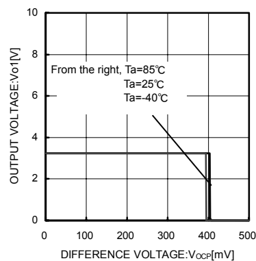
Fig.11 OCP Detection Voltage
