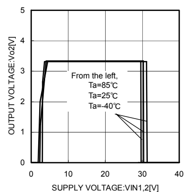
Fig.6 Vo2 Line Regulation
