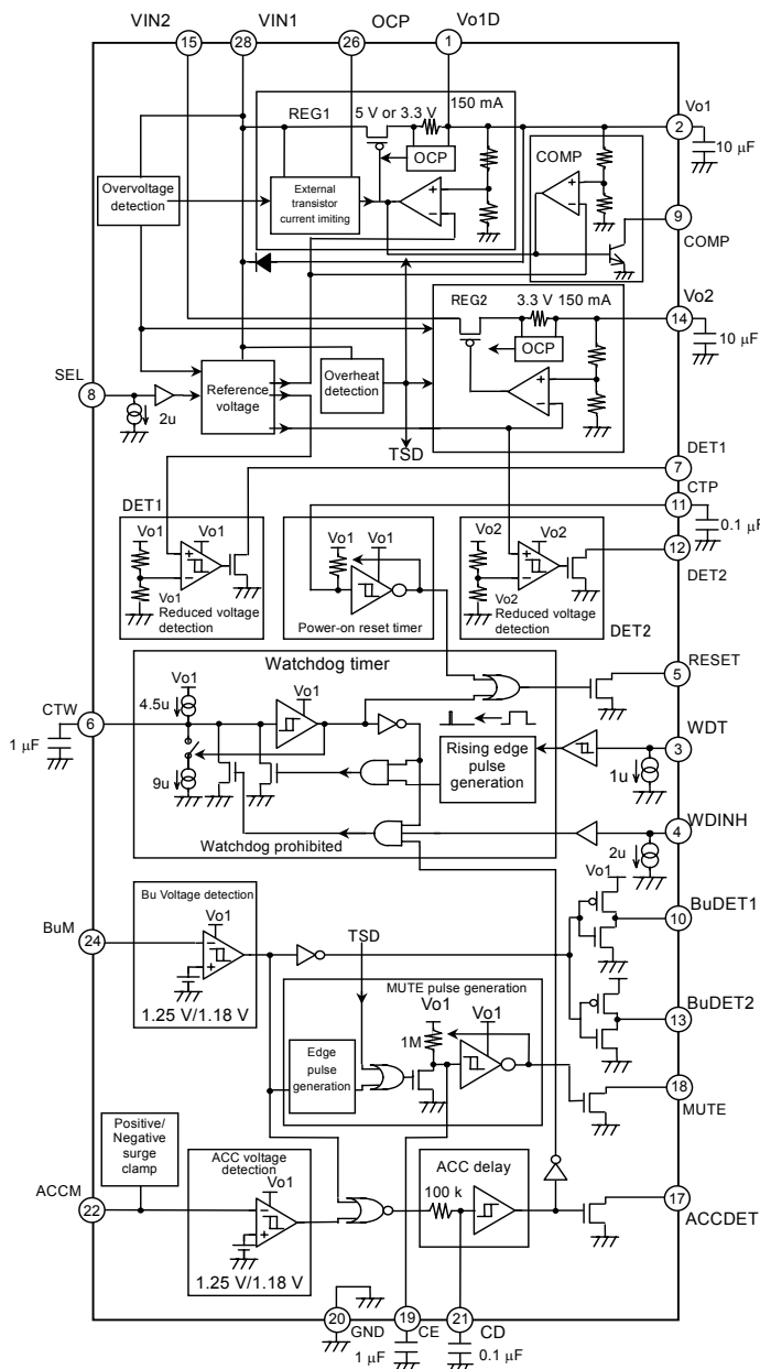
Fig.49 Block Diagram
