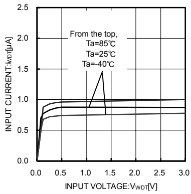
Fig.37 WDT Input Current 1 (SEL = L)
