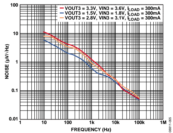
Figure 48. LDO2 Noise Spectrum Across Output Voltage, V_{IN} = V_{OUT} + 0.3\text{ V}
