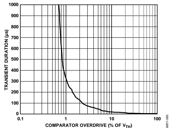
Figure 64. Maximum V_{\text{TH}} Transient Duration vs. Reset Threshold Overdrive
