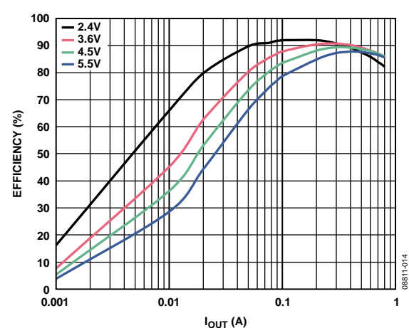
Figure 14. Buck Efficiency vs. Load Current, Across Input Voltage, V_{OUT2} = 1.8\text{ V} , PWM Mode
