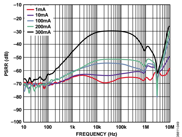
Figure 50. LDO2 PSRR Across Output Load, V_{IN3} = 3.3\text{ V} , V_{OUT3} = 2.8\text{ V}
