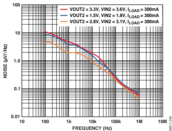
Figure 47. LDO1 Noise Spectrum Across Output Voltage, V_{IN} = V_{OUT} + 0.3\text{ V}
