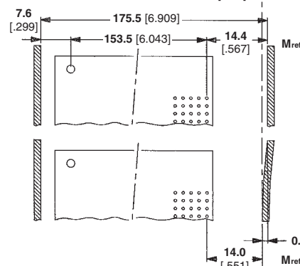
Subrack tolerances
