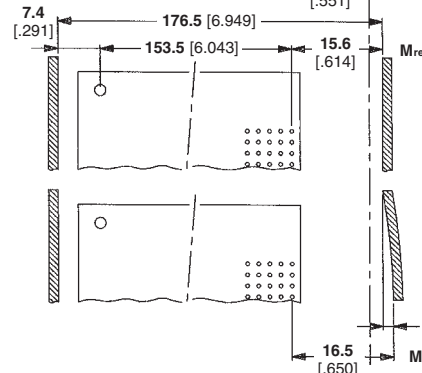
Allowed Misalignment, Transverse & Longitudinal Axes
