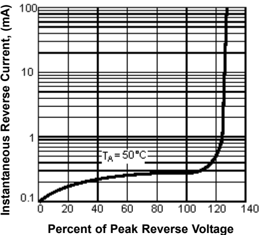
Figure 3 -Typical Peak Reverse Characteristics
