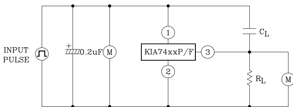
TEST CIRCUIT 2.
