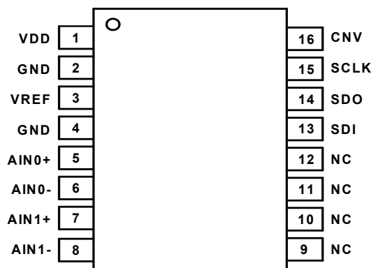
ISL26312 (16 LD TSSOP) TOP VIEW
