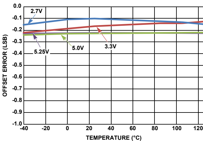
FIGURE 8. OFFSET ERROR vs SUPPLY VOLTAGE AND TEMPERATURE
