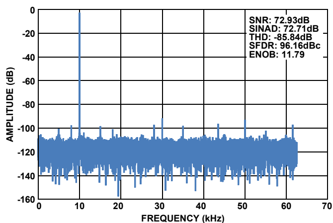
FIGURE 17. SINGLE-TONE FFT
