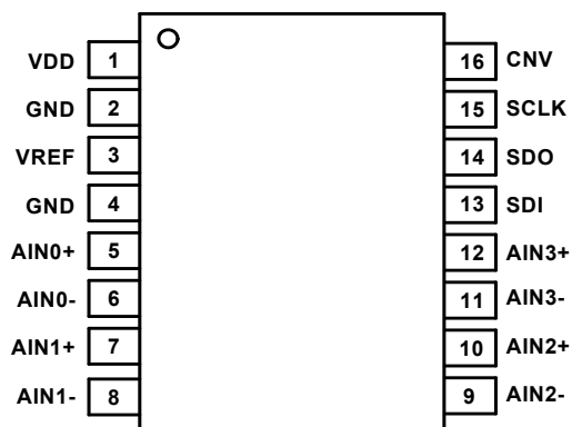
ISL26314 (16 LD TSSOP) TOP VIEW
