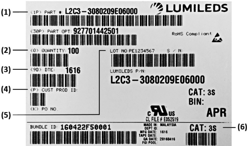
Figure 10. Example of inner box label for LUXEON SunPlus CoB Line.
