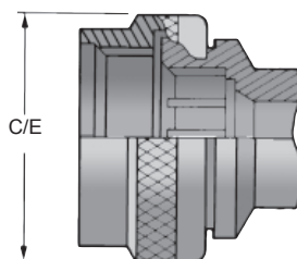
MIL-C-28840 FIGURE 7
