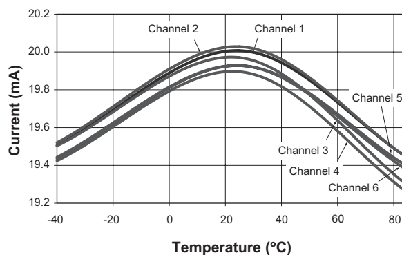
Current Matching vs. Temperature
