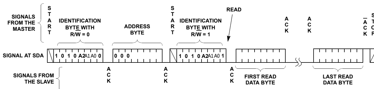
FIGURE 30. READ SEQUENCE
