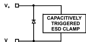
CIRCUIT 3
