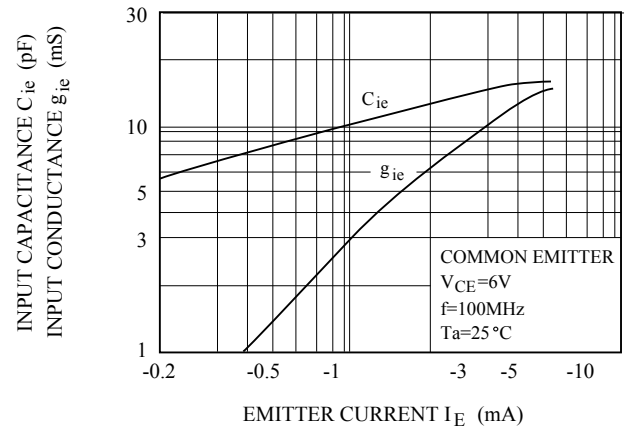
C_{ie}, g_{ie} - I_E
