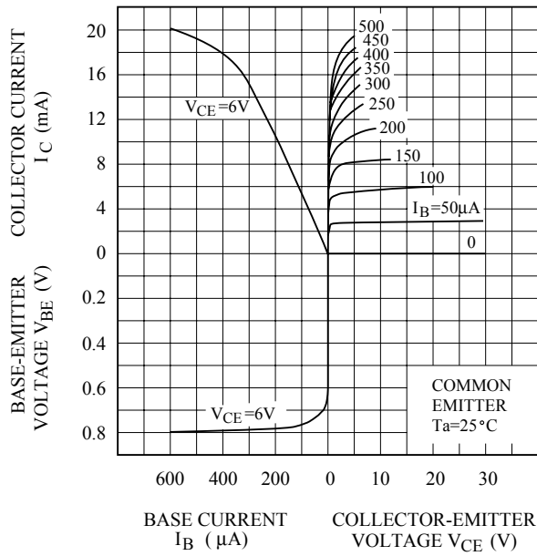
STATIC CHARACTERISTICS
