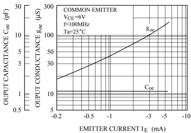
C_{oe}, g_{oe} - I_E
